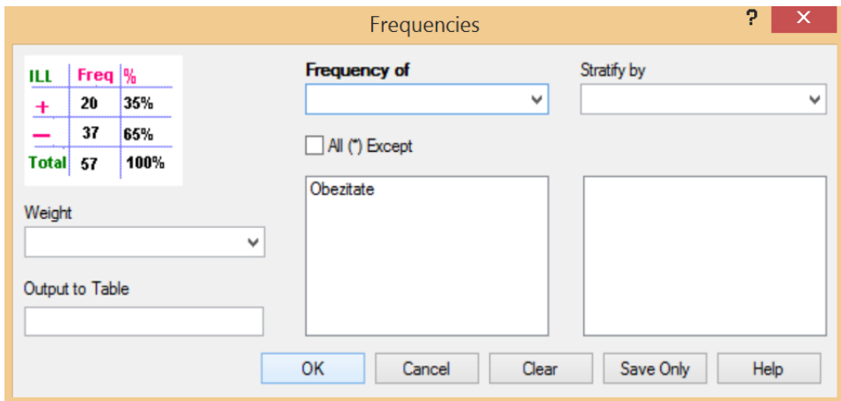
Figura 4. Aplicarea comenzii Statistics → Frequencies .
